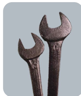
Mandrel wrenches R231-232-233-234 Part No. 460 000 423
